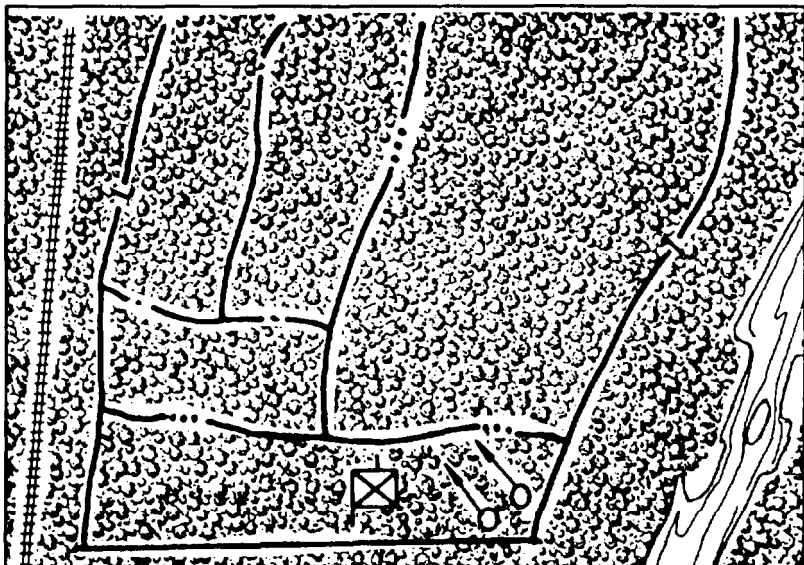
Figure 1-3 Assigned sectors.
